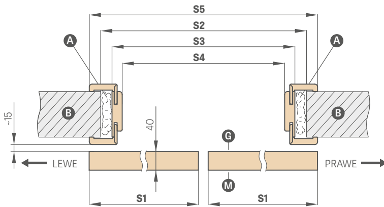
SP2N (obverse version)
