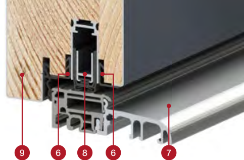
cross-section of the THERMO 64 leaf with and without drop down gasket, aluminium threshold
