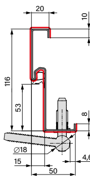
CORNER STEEL FRAME
